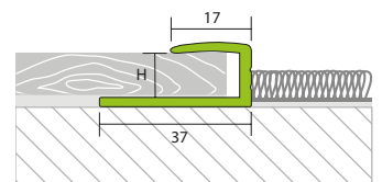
Höhe 12-14 mm / 14-16 mm
