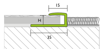
Höhe 7-9 mm / 9-11 mm
